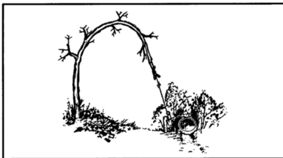
Figure 8-7. Twitch-up snare.
