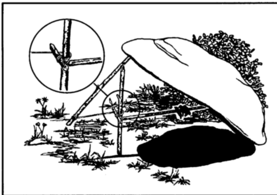
Figure 8-13. Paiute deadfall.
