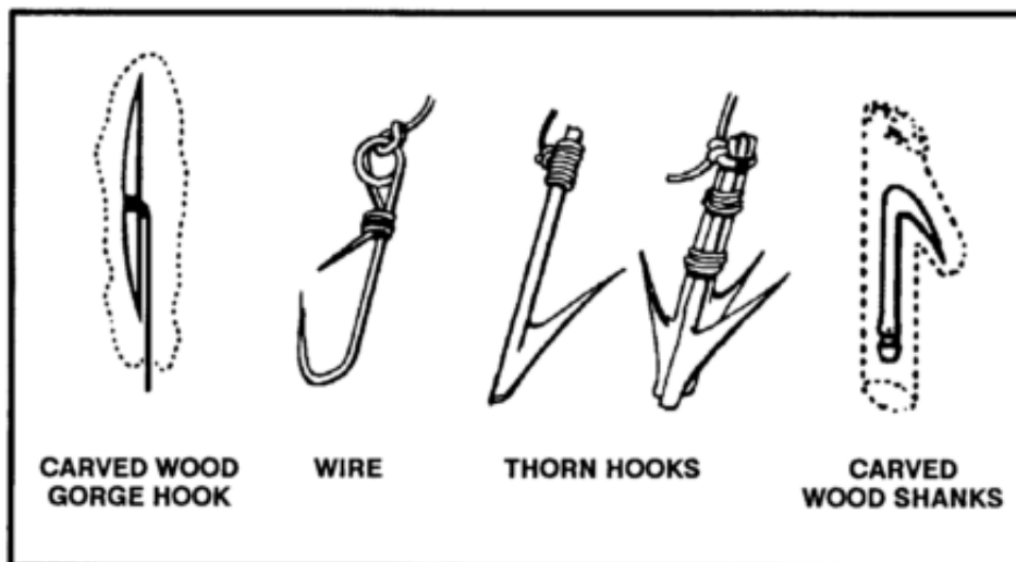
Figure 8-17. Improvised fishhooks.
