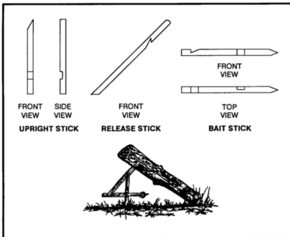
Figure 8-12. Figure 4 deadfall.
