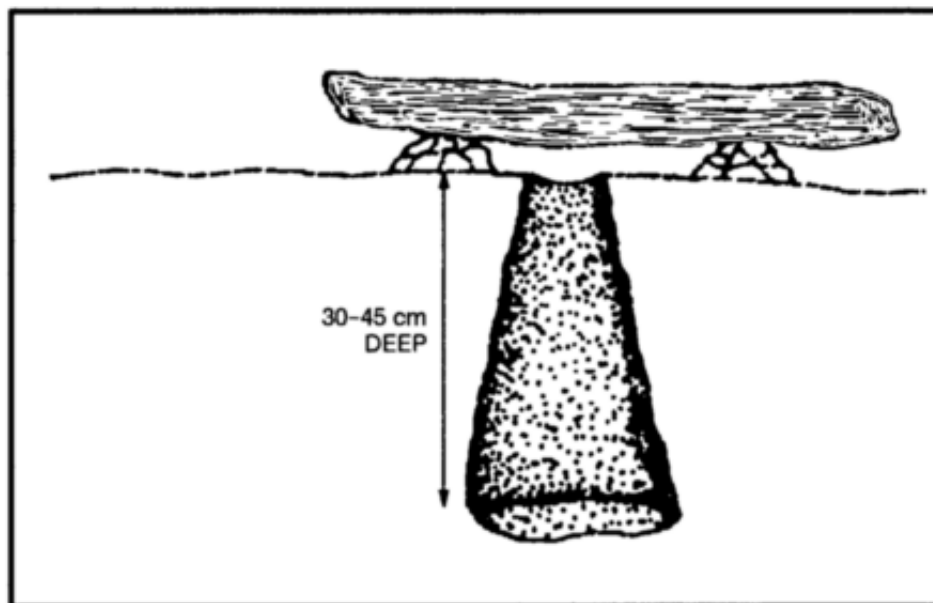
Figure 8-16. Bottle trap.
